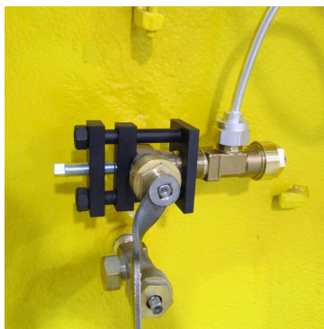
IVH-100-500 mounted on a ton container with flexible connector.
