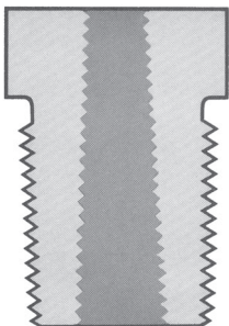
Figure 3 – Fusible Plug
