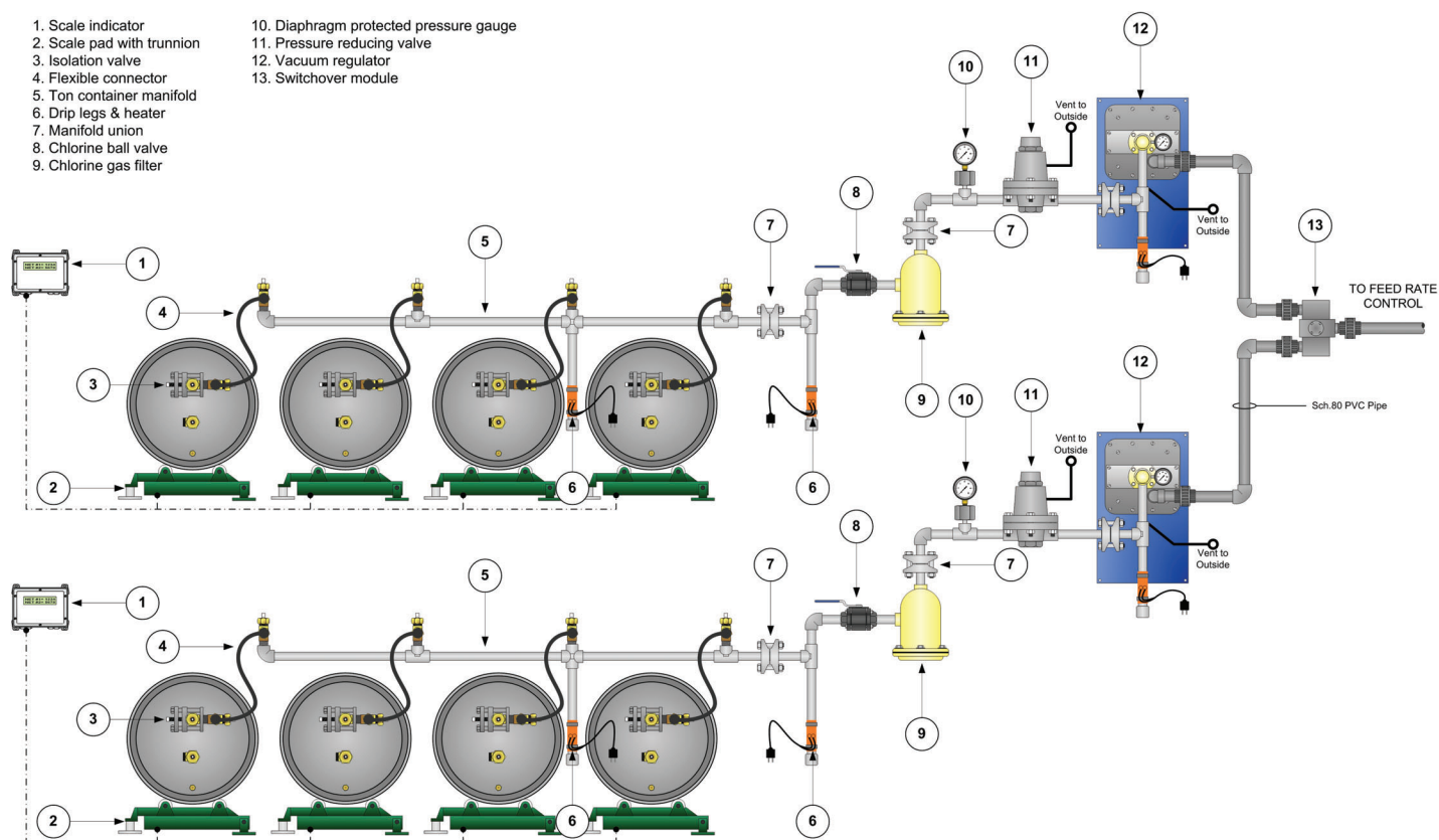
Figure 7 – Vacuum Switchover System
